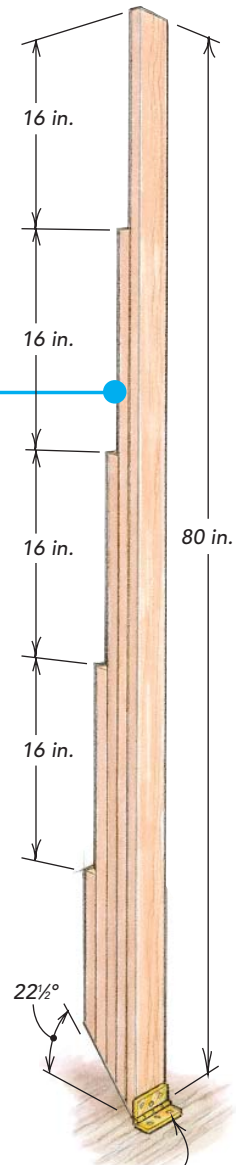
A 3-in. butt hinge is screwed to the floor and the fixture.
