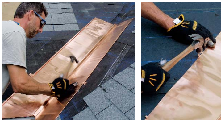
Two ways of holding down the liner. To allow the liner to expand lengthwise, fasteners cannot be driven through the liner. Instead, nails can be driven snug along the edge of the liner (photo right), or simple clips can engage a hem along the edge (photo left).
