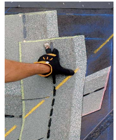
Insert a tab to stretch the course. Every course should wrap through the valley with a full shingle. A single- or a double-tab shingle may be installed to allow the shingle to extend through the valley (photo left) a minimum distance of 8 in., or the distance from thumb to middle finger (photo right).
