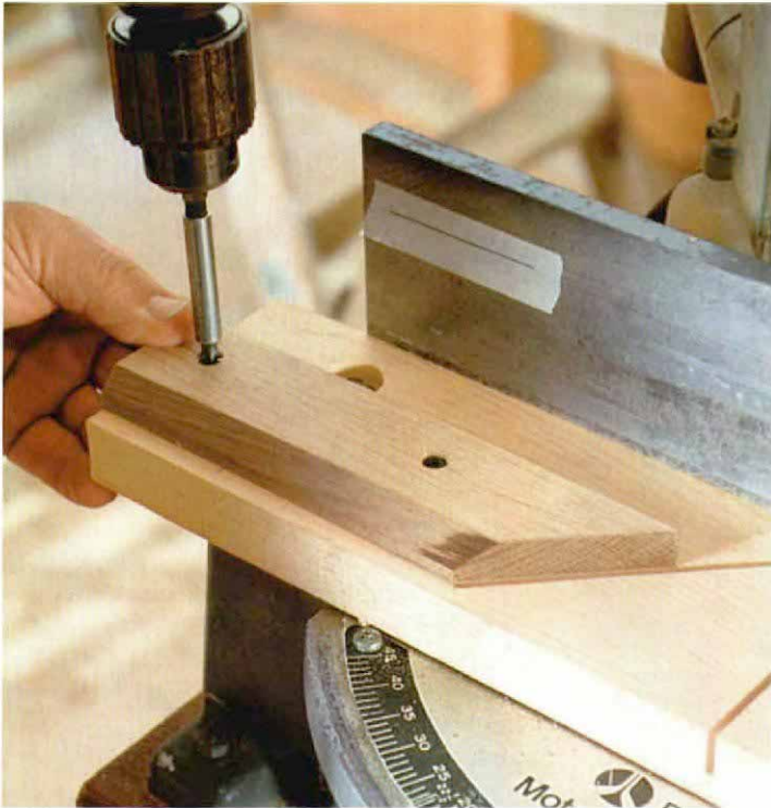
Miter-saw jig keeps correct spring angle. With the gauge block used to mark the crown height on the backing trim, the author transfers a mark to a piece of masking tape applied to the fence (photo top left). This mark corresponds to the mark on the wall measured by the gauge block. Holding a piece of molding upside down against the mark on the fence, the author transfers the molding's angle to the table (photo above). A length of scrap wood keeps the molding's angle proper (photo bottom left).
