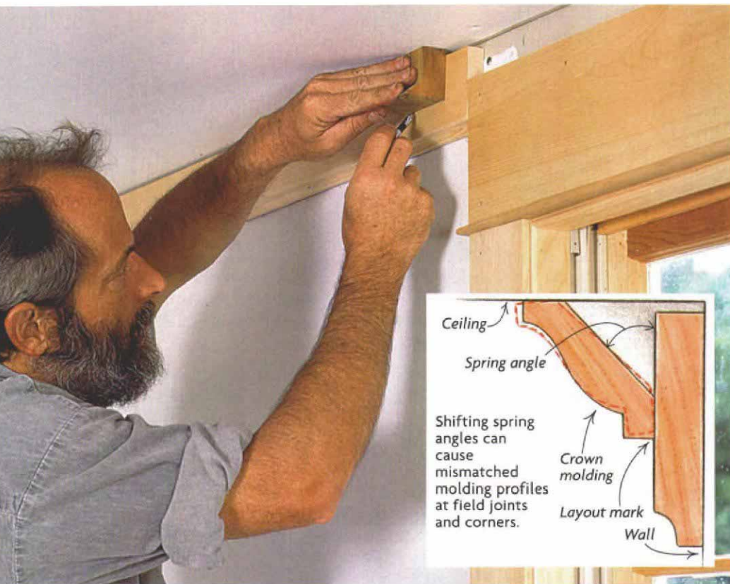
Gauge block shows exactly where the bottom of the molding must lie. Layout marks keep molding at a consistent angle to the wall, which in turn makes miters and field joints line up.
