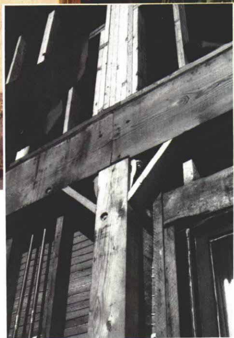
An independent post-and-beam skeleton. Lag-bolted to the first-floor framing, 4x8 posts rest on individual piers (drawing and photo, left). Atop the posts, 4x16 beams form a structural perimeter to hold floor joists and walls of the second story (inset, above). The badly deteriorated original stucco finish has been removed from the first-floor walls (top). They will be restuccoed. The exterior on the new second story will be board and batten.
