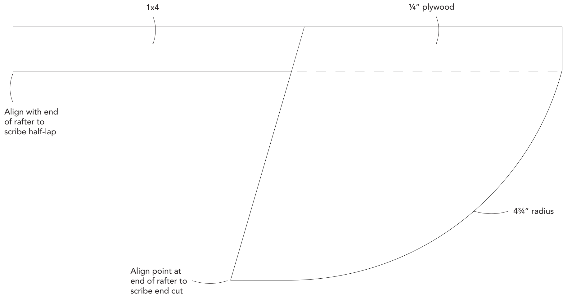
Full-size rafter jig
